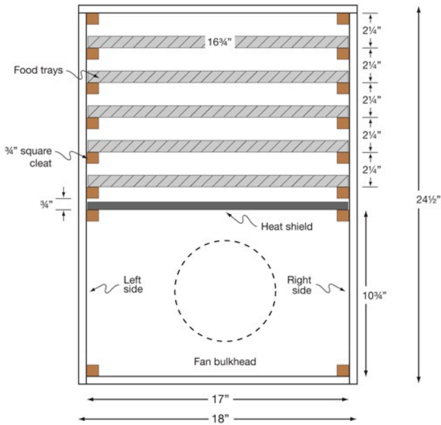
Figure 3. Front view cross-section of dehydrator construction
