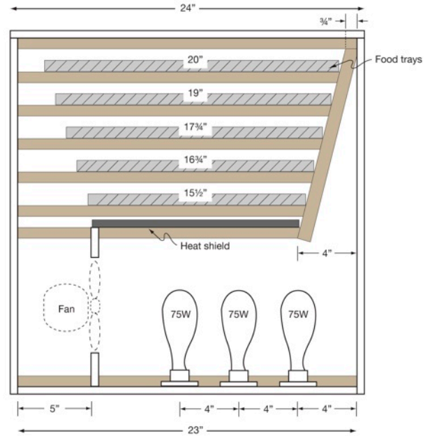
Figure 4. Side-view cross-section of dehydrator construction
