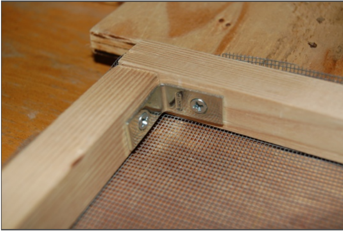
Figure 10. “L-bracket” used to re-inforce corners of drying trays
