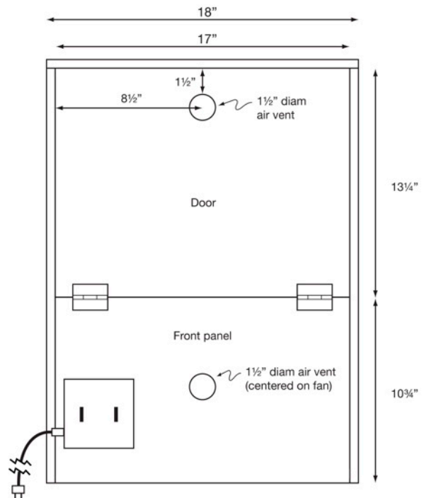
Figure 2. Front view of dehydrator construction.
