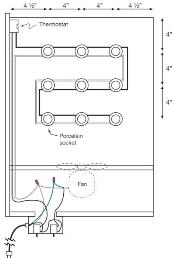
Figure 6. Layout of sockets and wiring plan
